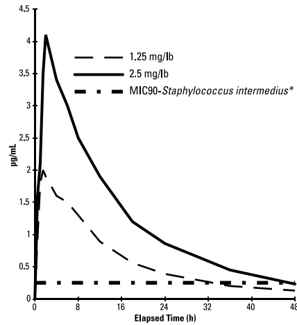
Figure 3: Mean plasma concentrations (µg/mL) following single oral administration of marbofloxacin to adult cats at a dosage of 2.5 mg/lb.
