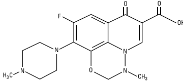
Figure 1: Chemical structure of marbofloxacin
