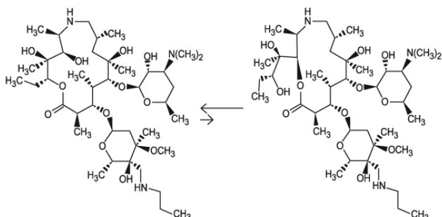
Figure 1. Tulathromycin structures
